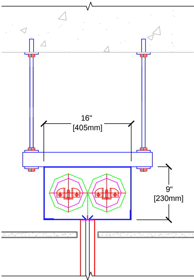
SIDE BY SIDE ROLLER HEADBOX
