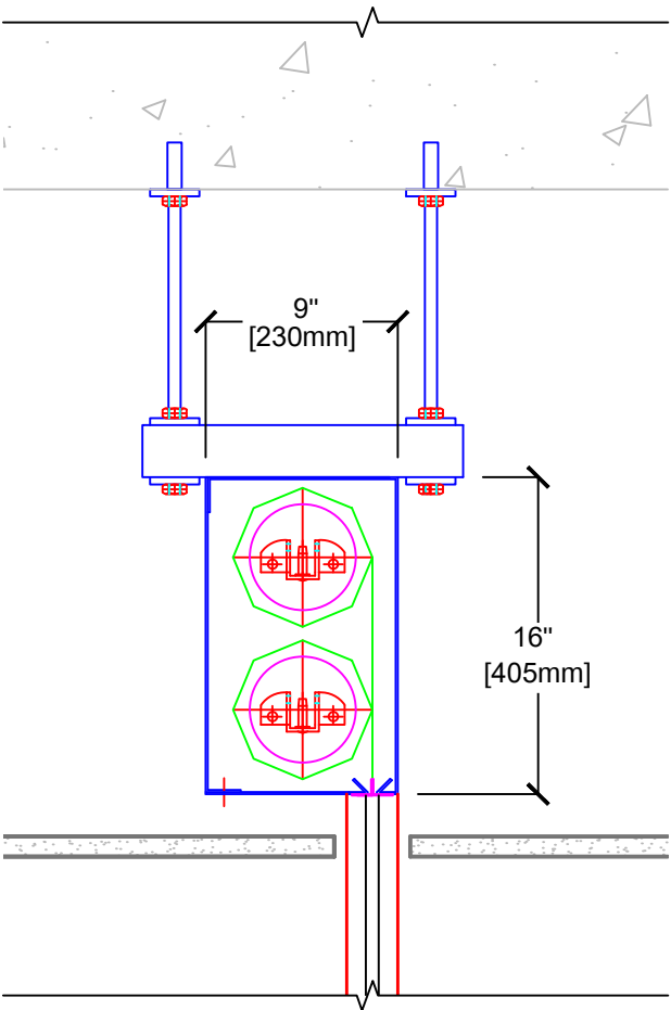
OVER-UNDER ROLLER HEADBOX
