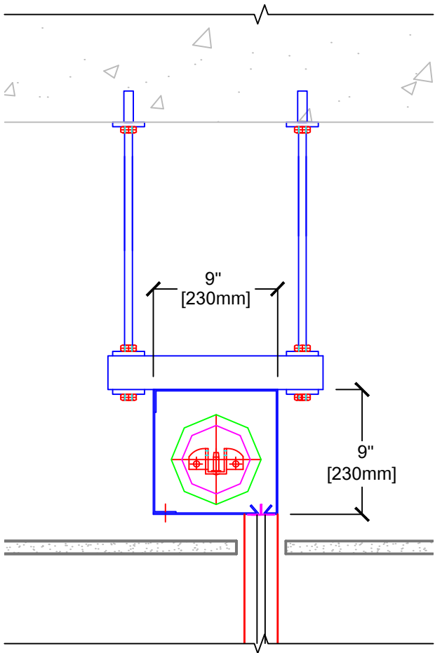
SINGLE ROLLER HEADBOX
