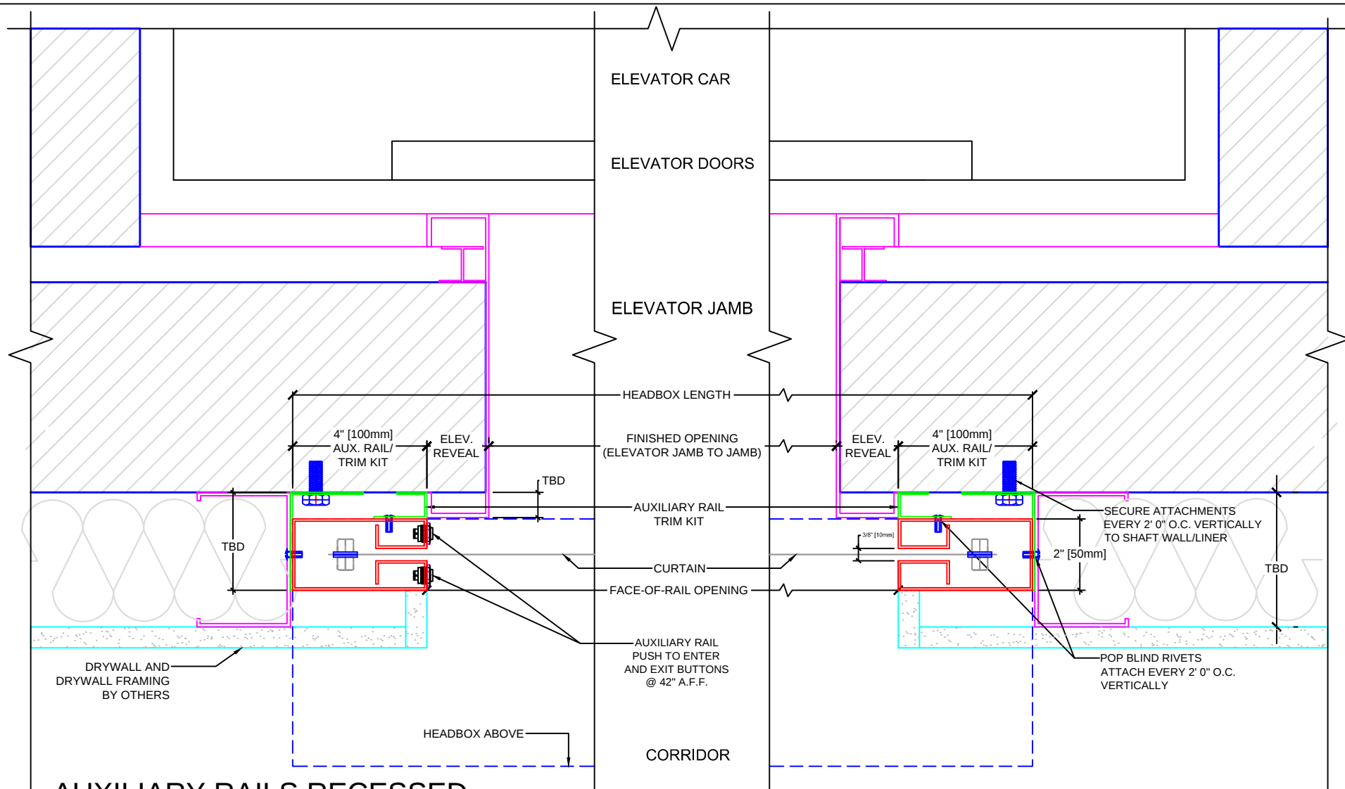
AUXILIARY RAILS RECESSED OFFSET BESIDE ELEVATOR FRAME REVEAL OPTION A (NOT PROJECT SPECIFIC)
