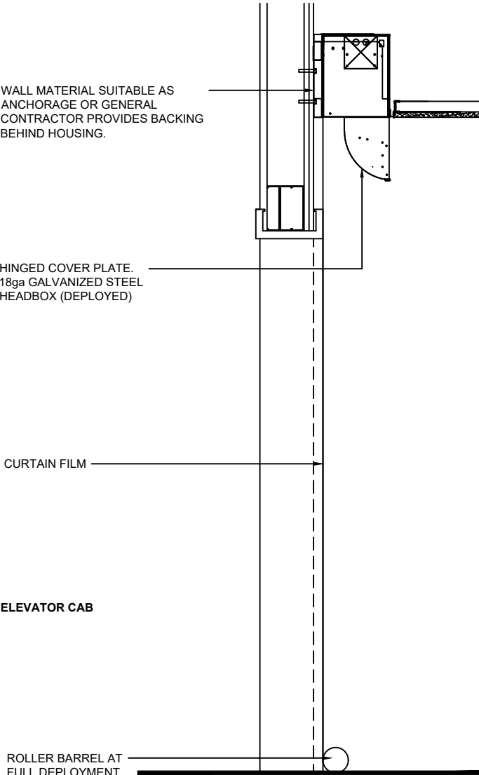
SECTION OF ELEVATOR - CURTAIN FULLY DEPLOYED TO FLOOR
