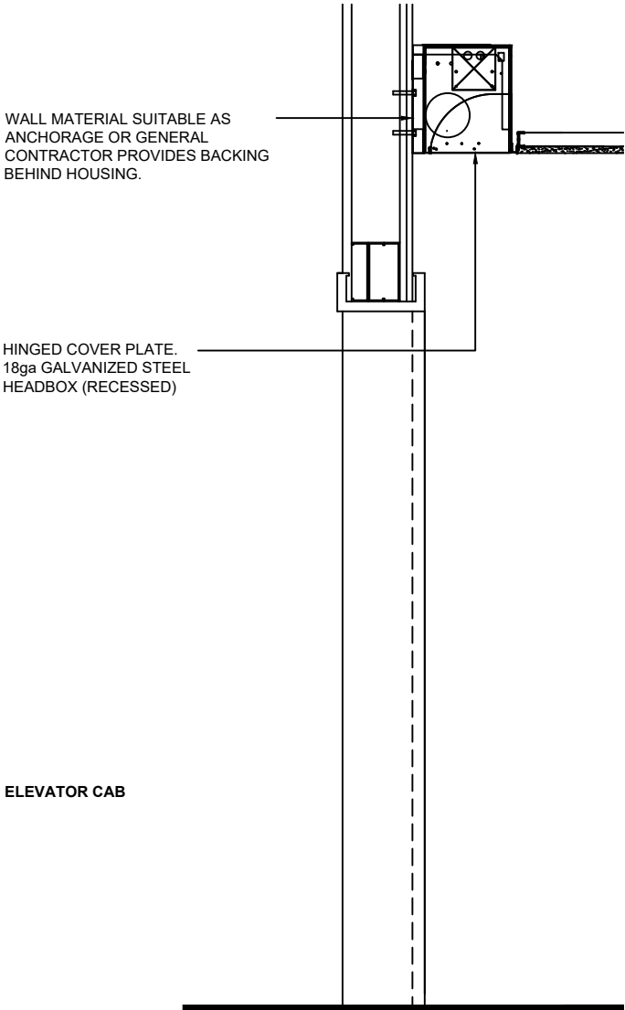
SECTION OF ELEVATOR - CURTAIN NOT DEPLOYED
