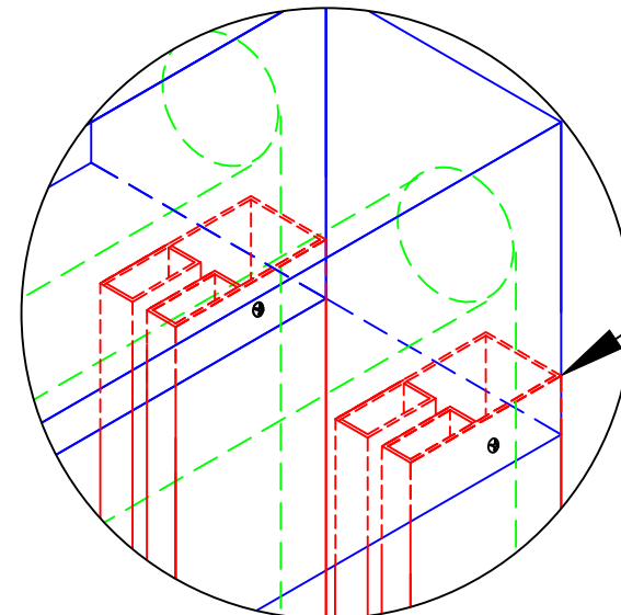
ENLARGED MOUNTED SIDE GUIDE DETAIL SIDE GUIDES TO EXTEND UP TO INTERNAL BOX STOP BRACKET. RIVET AT SIDE AND BACK OF RAIL THROUGH BOX.
