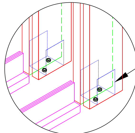
ENLARGED FLOOR BRACKET DETAIL TWO BOLTS INSTALLED THROUGH BRACKET TO FLOOR
