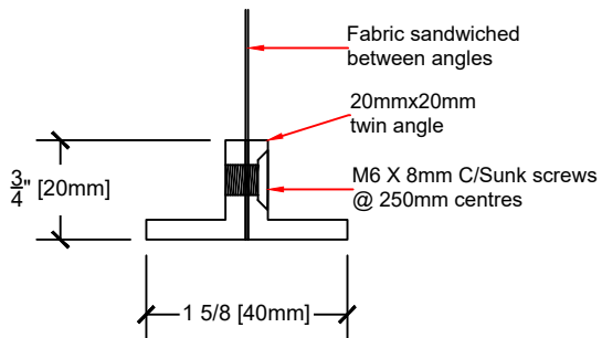
STANDARD BOTTOM BAR
