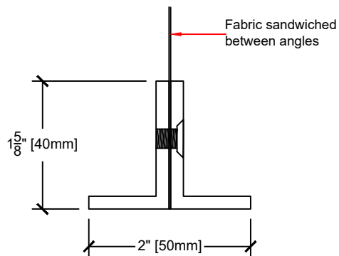
HEAVY BOTTOM BAR
