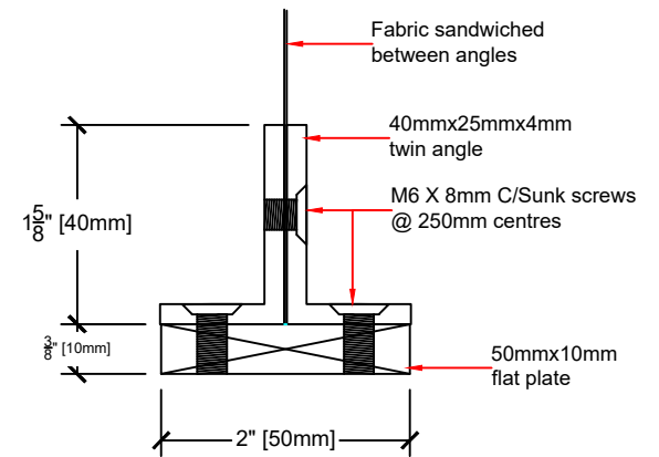
HEAVY BOTTOM BAR WITH FLAT
